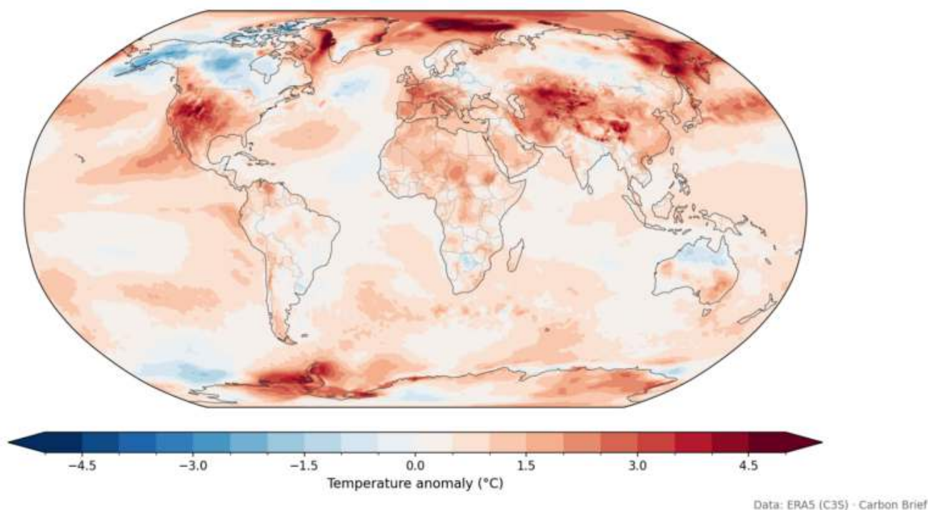
January-June 2026 near-surface air temperature anomaly ERA5 relative to 1981-2010 baseline
