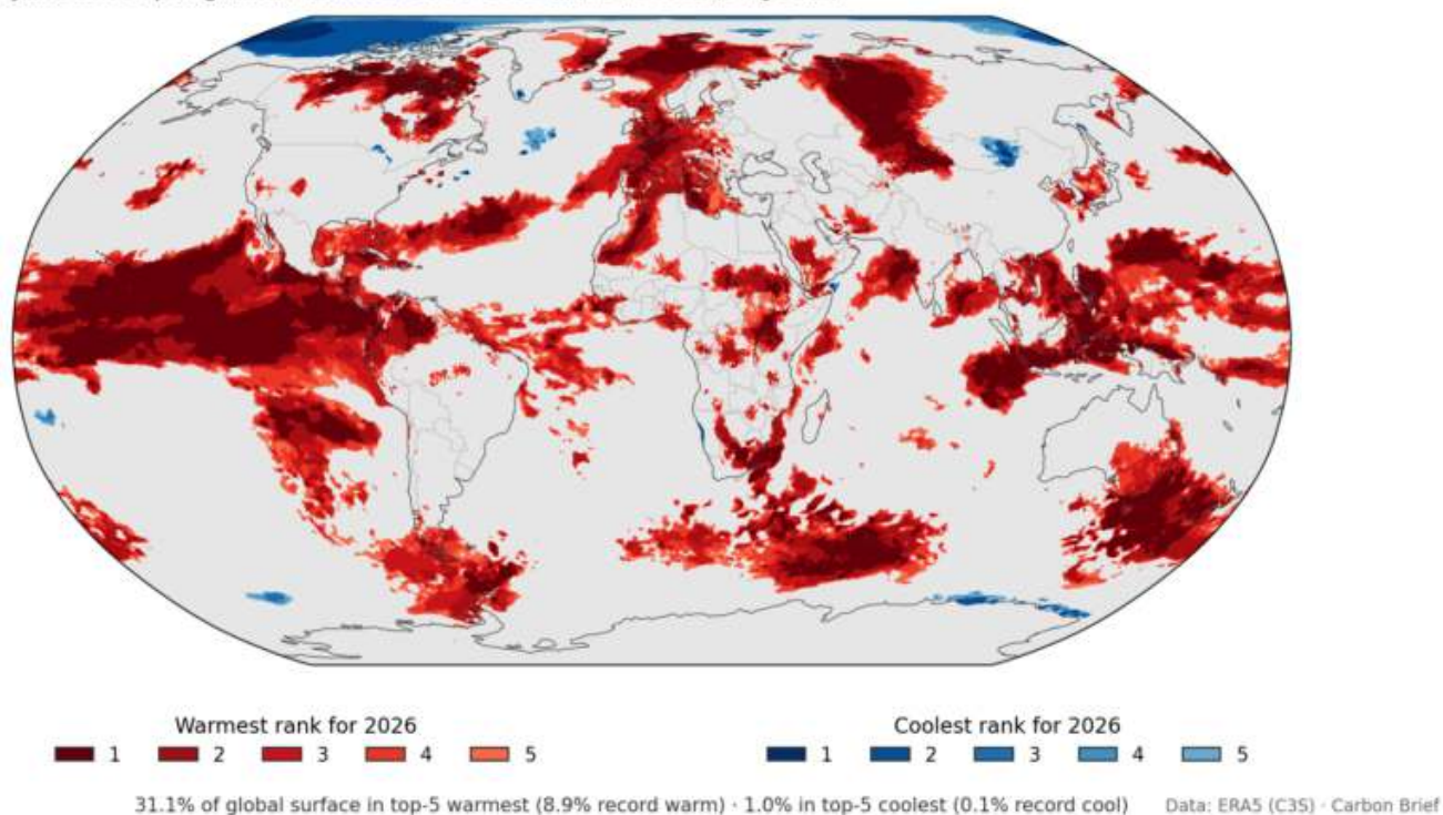
June 2026: per-gridcell rank vs. 1940-2026 ERA5 record (87 years)
